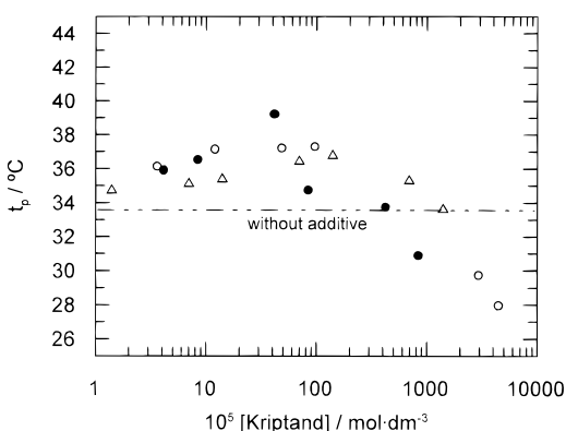
Figure 4. Variation of A from eq 1 ( t_p ) with cryptand concentration: (Δ) C211; (●) C221; (○) C222.
